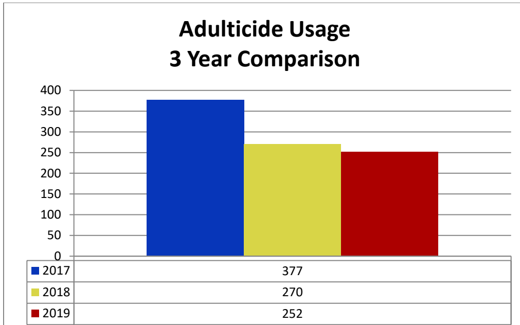
Figure 7. 3-year comparison of adult mosquito control products used in the GCMAD.
