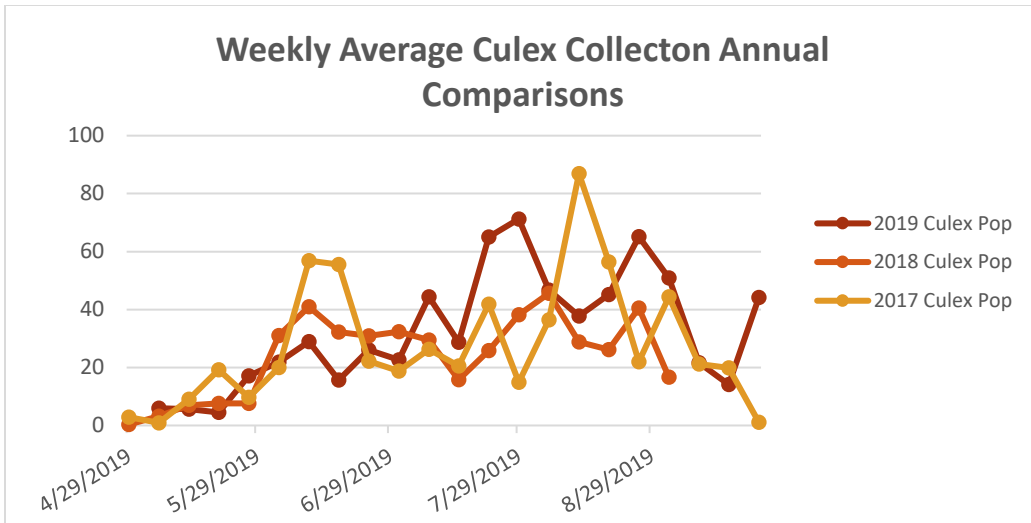
Figure 3. District-wide three-year weekly average Culex collections.
