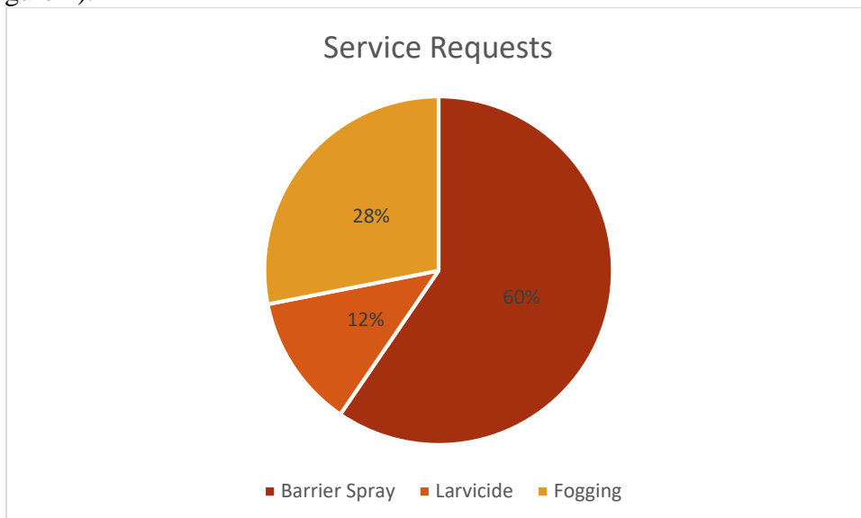
Figure 4. District-wide service requests received in 2019.
