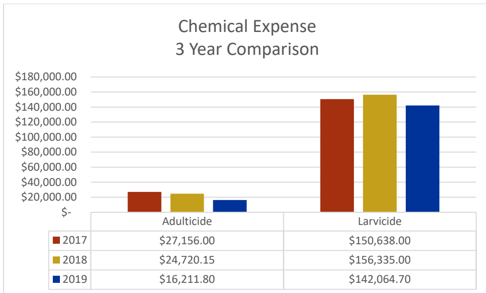
Figure 10. Three year comparison of product costs for the GCMAD.
