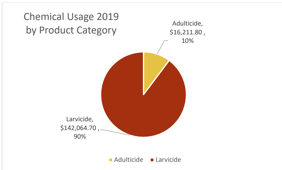
Figure 9. The amount of money spent on larvicide and adulticide products and the proportion of product budget spent on each category.
