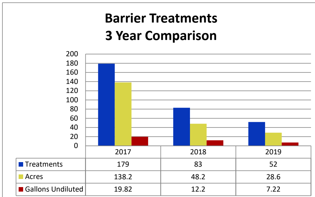
Figure 8. 3 year comparison of barrier treatments by GCMAD.
